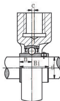
SR type seal
